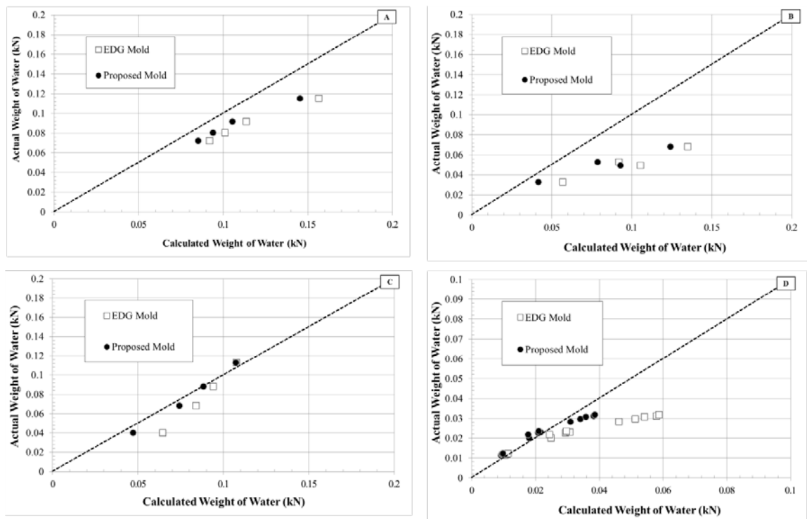
Figure 2.8: Weight of water performance results for (A) Fayette County clay, (B) Davies County clay, (C) Lee County clay, and (D) Gallatin County sand
