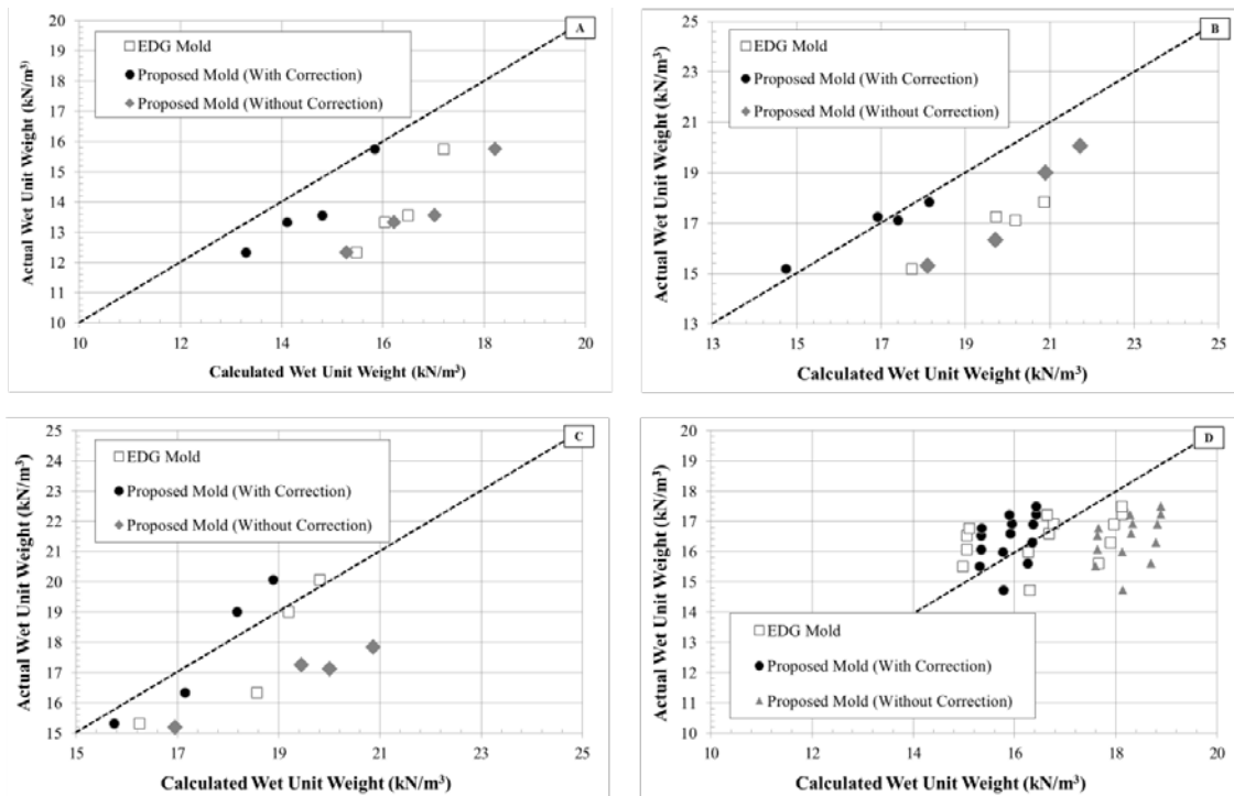
Figure 2.9: Wet unit weight model performance results for (A) Fayette County clay, (B) Davie County clay, (C) Lee County clay, and (D) Gallatin County sand
